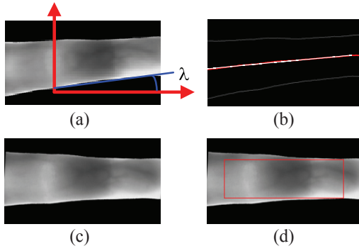
Figure 8. Finger displacement adjustment and ROI localization. (a) Original image; (b) Synthesized line (in red); (c) Adjusted image; (d) Localized ROI (in red rectangle).
