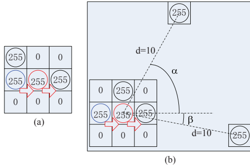
Figure 5. Tracking criteria. (a) Not backtrack; (b) Neighbor point with the smaller angle first. The blue circle means the tracked point; the red one is the current point; the black ones are neighbor points of the current point. And the red arrow means the tracking direction.
